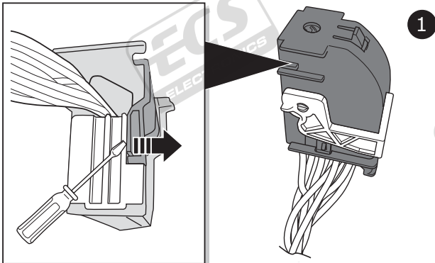
Black Connector 32 pole
