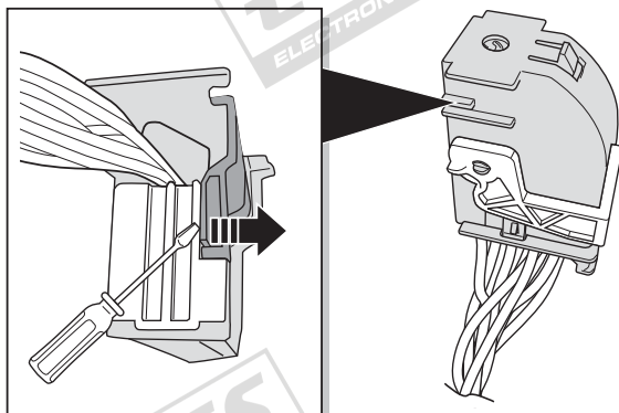
Blue Connector 32 pole
